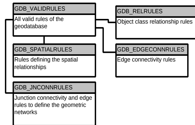
The geometric network edge/junction rules
